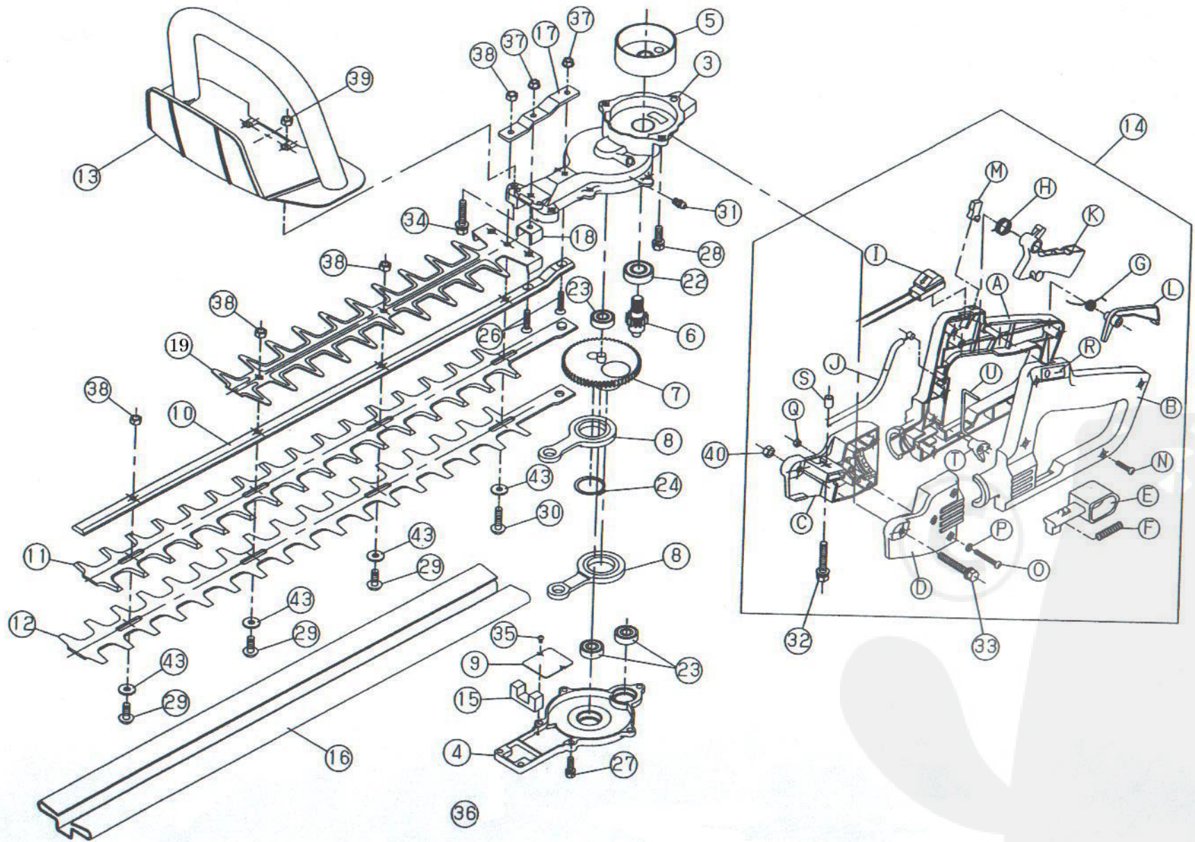
HEDGE TRIMMER MODEL HF600DT-PRO DEC. 01. 2003
