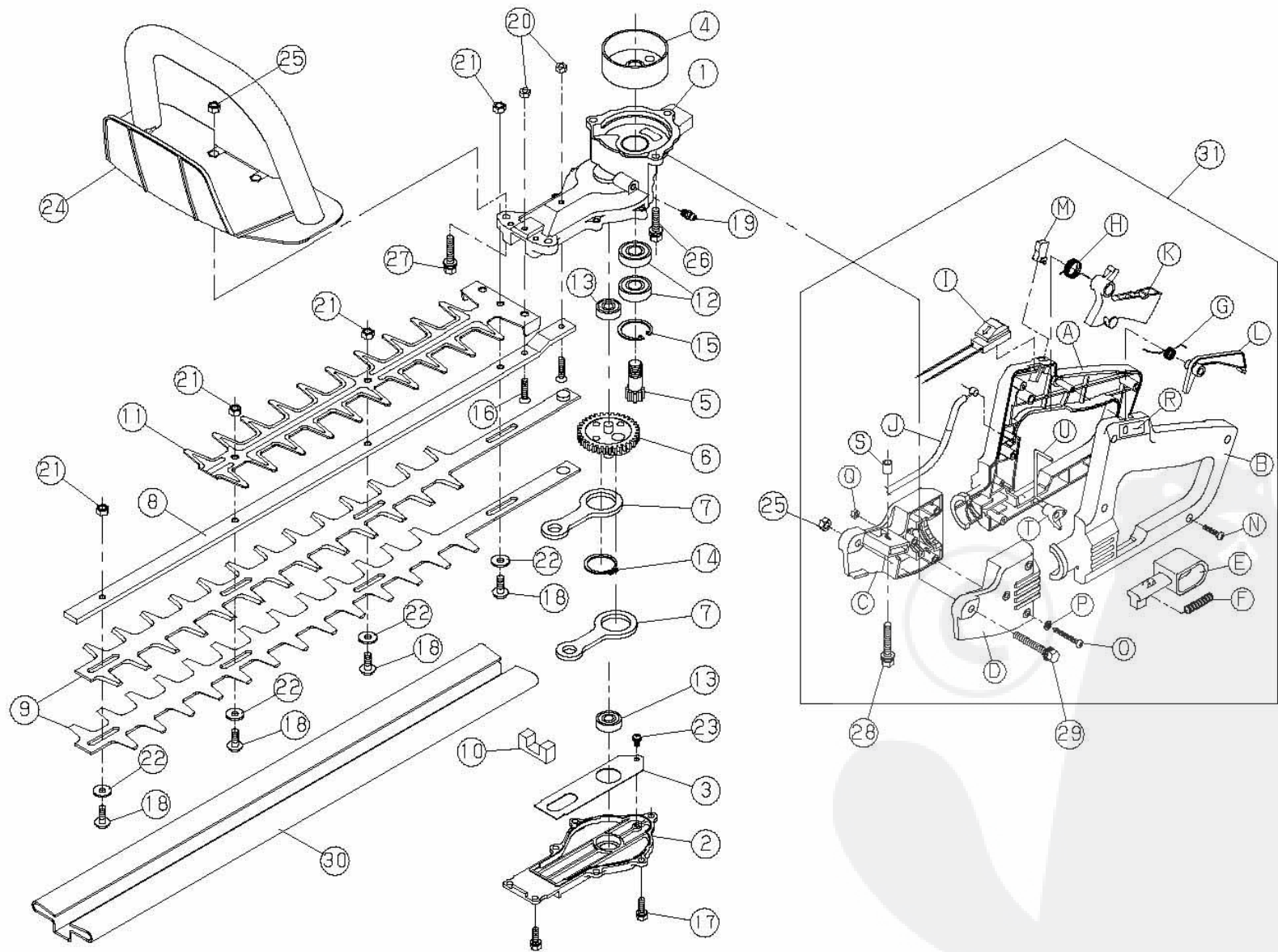
HEDGE TRIMMER MODEL HF550DT-L 0401
