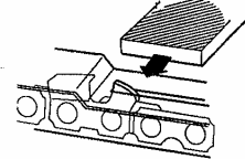
Using a Depth gauge joiner
