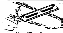
Use a Filing Gauge
