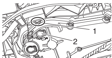
1. Grease fitting
