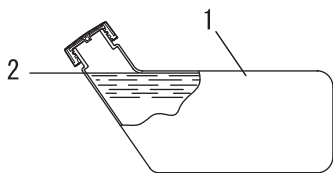
1. Fuel tank 2. Shoulder level
