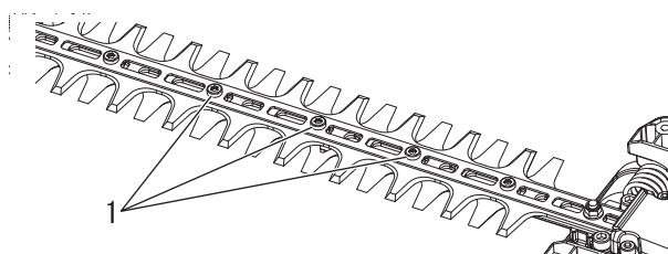
1. Shoulder bolt
