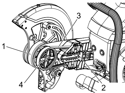
1. Snijarm 2. Starterbehuizing 3. Riem 4. Grote katrol
