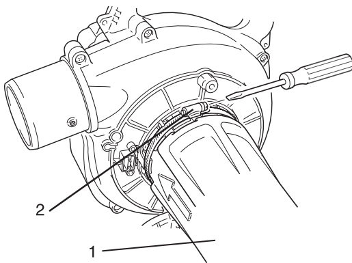
1. Vacuum tube
