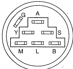
IGNITION SWITCH
