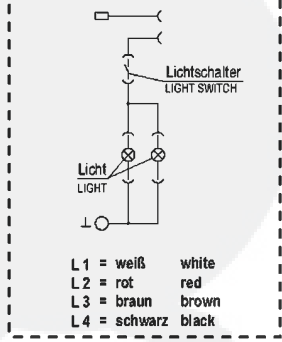
Schaltplan Licht CONNECTION DIAGRAM LIGHT
