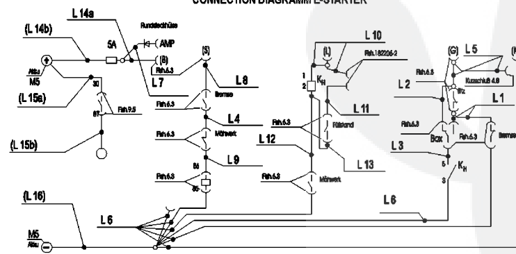
Schaltplan Traktor E-Start CONNECTION DIAGRAM E-STARTER
