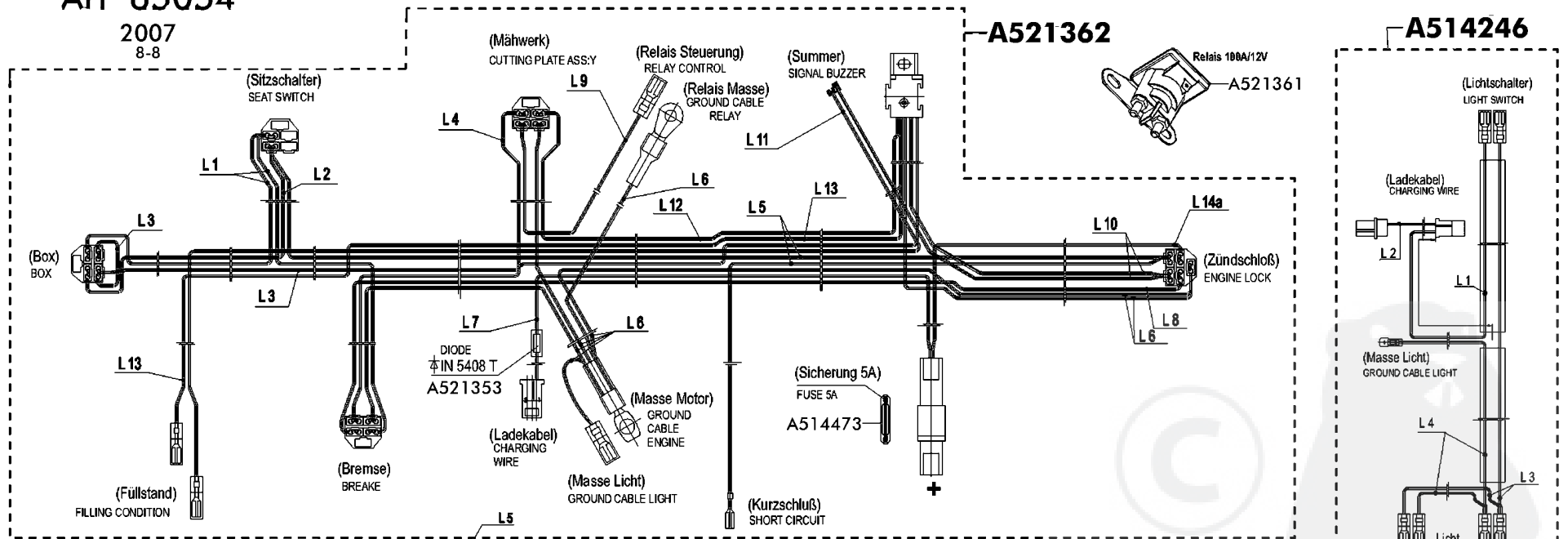
Schaltplan Traktor E-Start CONNECTION DIAGRAM E-STARTER
