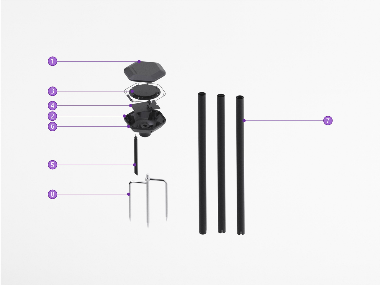
Disassembly diagram
